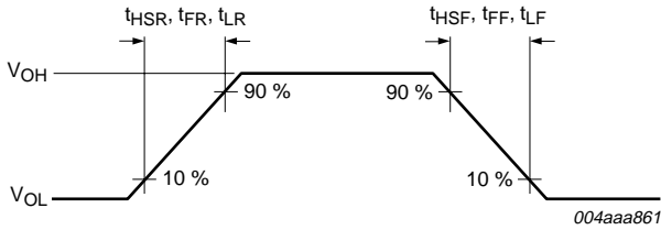
Fig 24. Rise time and fall time
